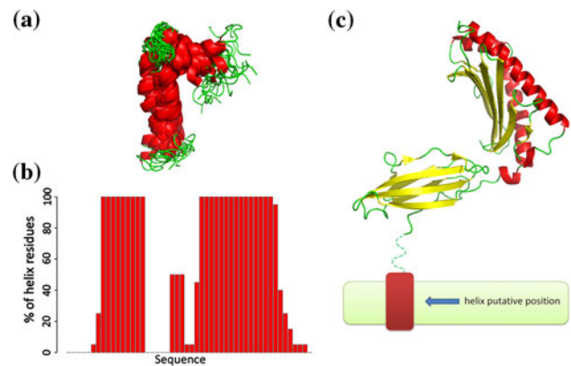
Fig. 1 Example of excluded proteins. a NMR models of membrane fd coat protein [PDB code 1FDM (Almeida and Opella 1997)]. b Protein HLA-B27 [PDB code 1HSA (Madden et al. 1992)] with putative transmembrane position
